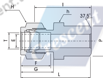
Male Pipe Weld Connector L-PCW
